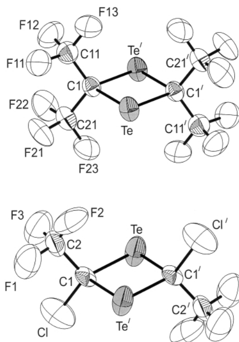
Fig. 1 Molecular structures and atomic labelling scheme of [(\text{F}_3\text{C})_2\text{C}=\text{Te}]_2 ( 4 ) (top) and [(\text{F}_3\text{C})(\text{Cl})\text{C}=\text{Te}]_2 ( 4a ) (bottom) with thermal ellipsoids shown at the 50% probability level.
